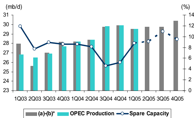
Graph 3: OPEC production versus spare capacity
